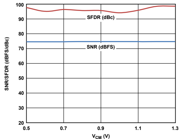
Figure 36. SNR/SFDR vs. Common-Mode Voltage; f_{IN} = 9.7 MHz, f_{SAMPLE} = 125 MSPS
