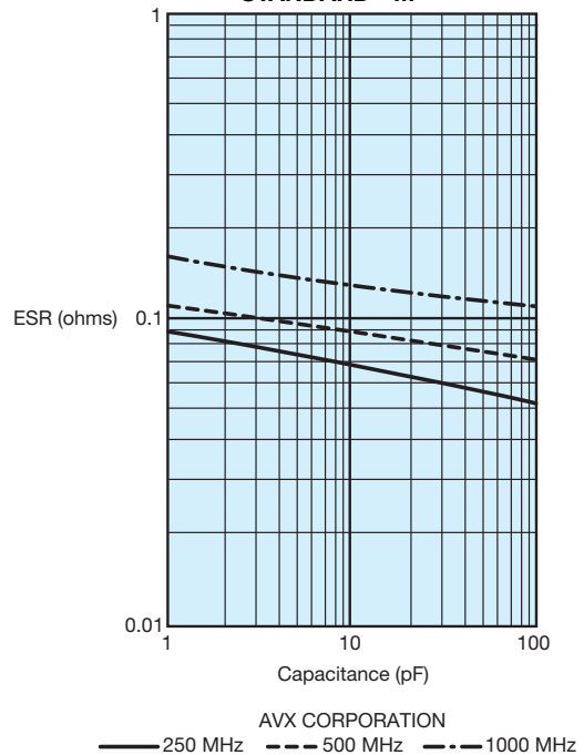
TYPICAL ESR vs. CAPACITANCE AQ11/12 MIL-PRF-55681E - BG STANDARD - M
