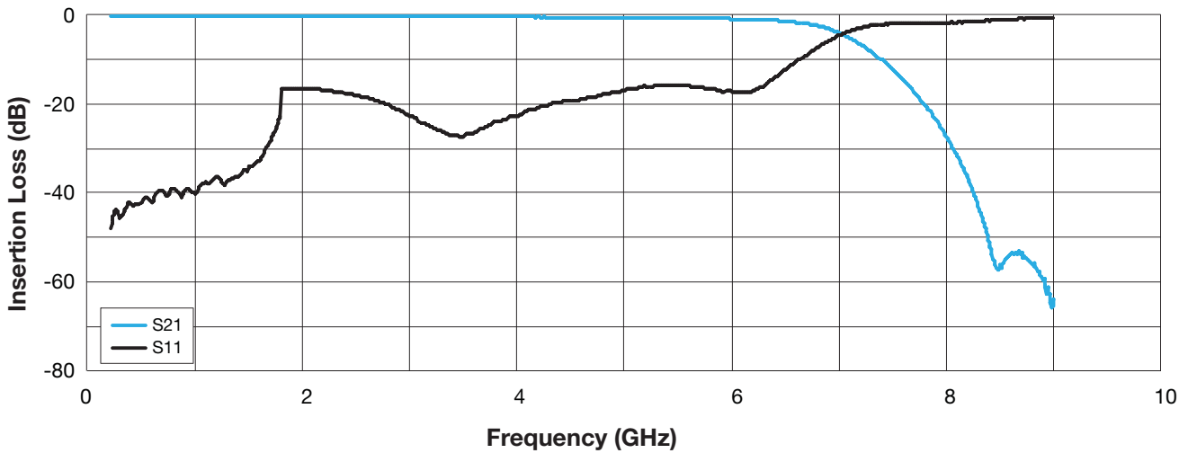
Typical Frequency Response
