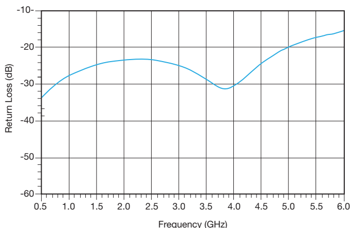
RF/DC Crossover – Return Loss
