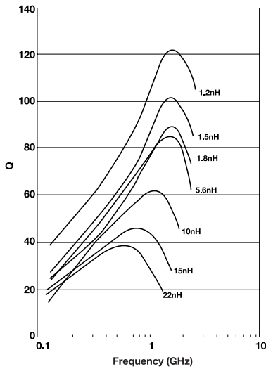
Measured on HP4291A and Boonton 34A Coaxial Line
