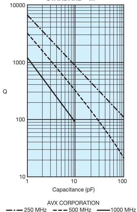
TYPICAL Q vs. CAPACITANCE AQ11/12 MIL-PRF-55681E - BG STANDARD - M
