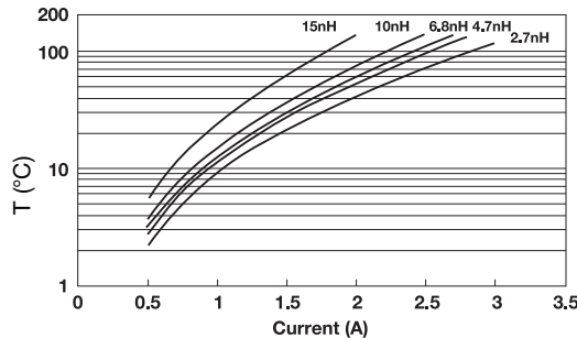
Temperature rise will typically be no higher than shown by the graph
