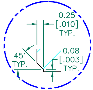
DETAIL "A" CHAMFER SCALE=12:1
