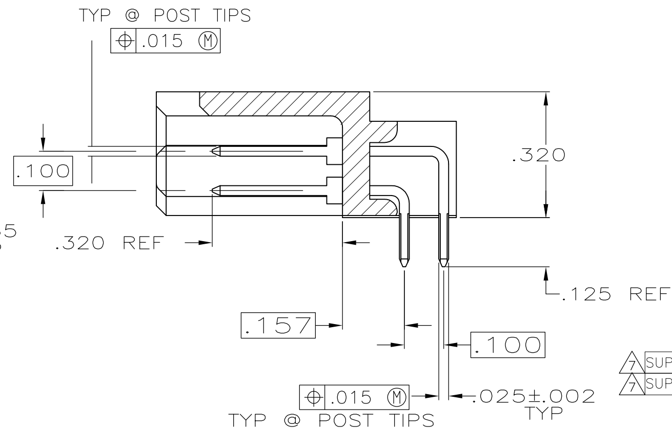
SECTION M-M
