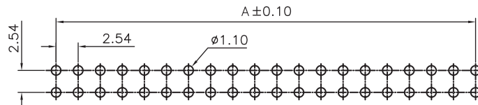
PCB LAYOUT - COMPONENT VIEW
