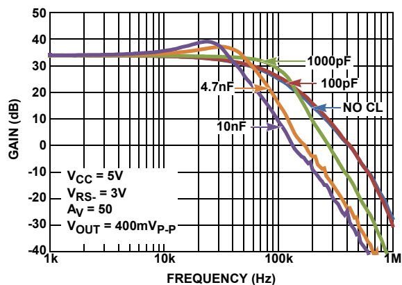
FIGURE 13. CAPACITIVE LOAD DRIVE GAIN vs FREQUENCY
