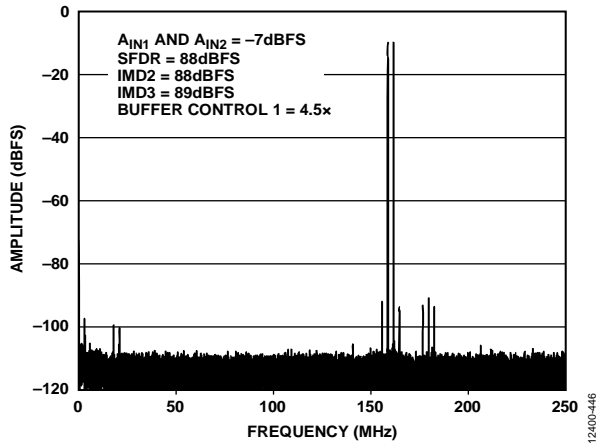
Figure 57. Two-Tone FFT; f_{IN1} = 338 MHz, f_{IN2} = 341 MHz
