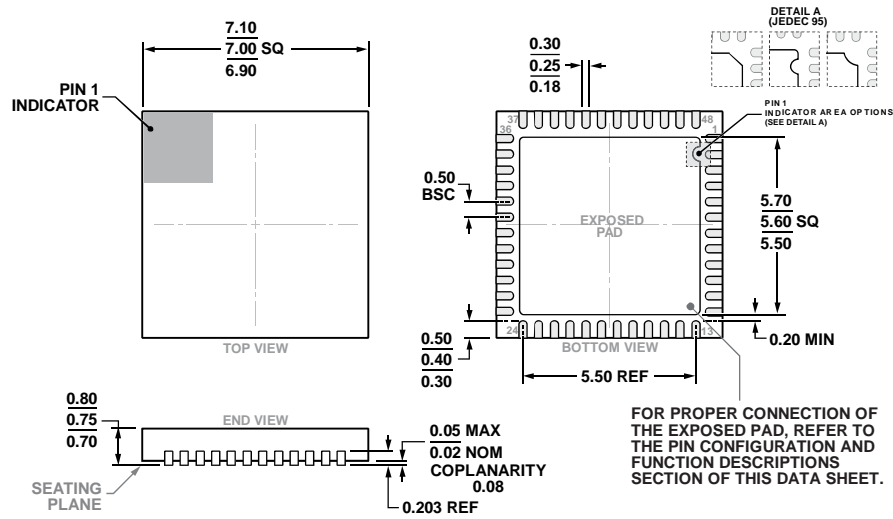
COMPLIANT TO JEDEC STANDARDS MO-220-WKKD-4. Figure 19. 48-Lead Lead Frame Chip Scale Package [LFCSP] 7 mm x 7 mm Body and 0.75 mm Package Height (CP-48-13) Dimensions shown in millimeters
