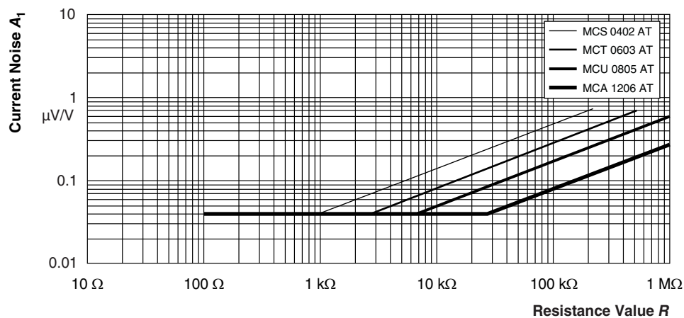
Current Noise
