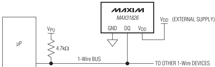
Figure 2. Powering the MAX31826 with an External Supply
