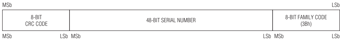
Figure 3. 64-Bit ROM Code
