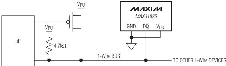
Figure 1. Supplying the Parasite-Powered MAX31826 During Temperature Conversions
