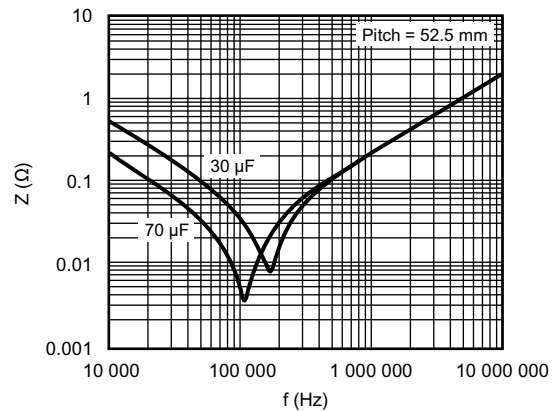
Impedance vs. frequency (typical curve)
