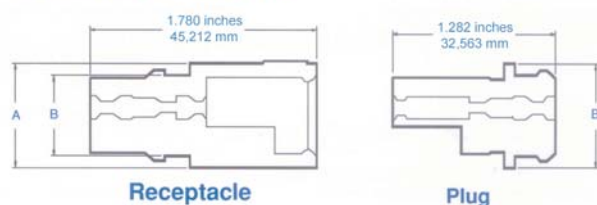
Low Insertion Force Type
