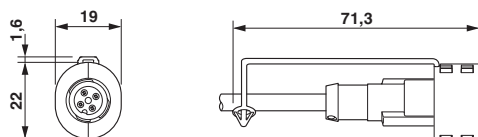
Dimensional drawing
