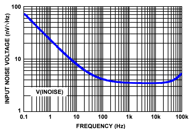
FIGURE 44. SIMULATED INPUT NOISE VOLTAGE
