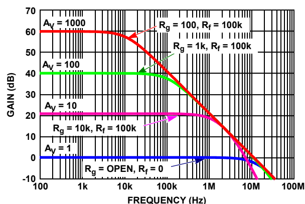
FIGURE 46. SIMULATED CLOSED LOOP GAIN vs FREQUENCY
