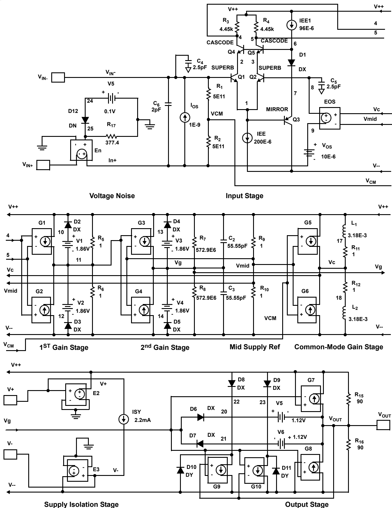
FIGURE 41. SPICE SCHEMATIC
