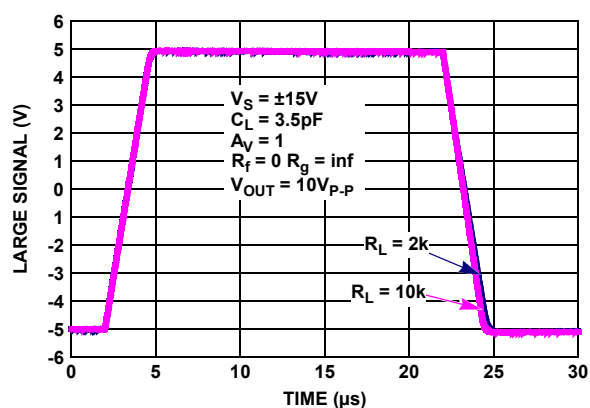
FIGURE 32. LARGE SIGNAL 10V STEP RESPONSE, V_S = \pm 15V
