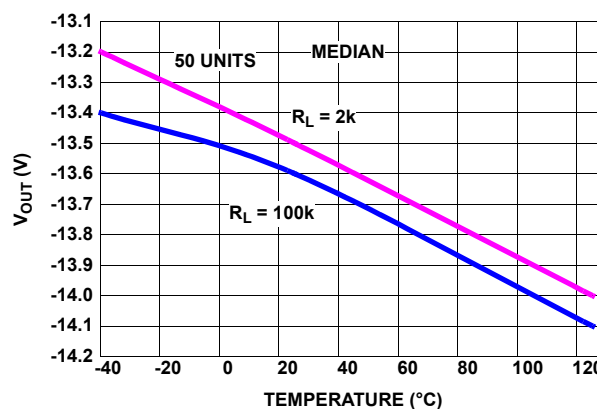
FIGURE 24. V_{OL} vs TEMPERATURE, V_S = \pm 15V
