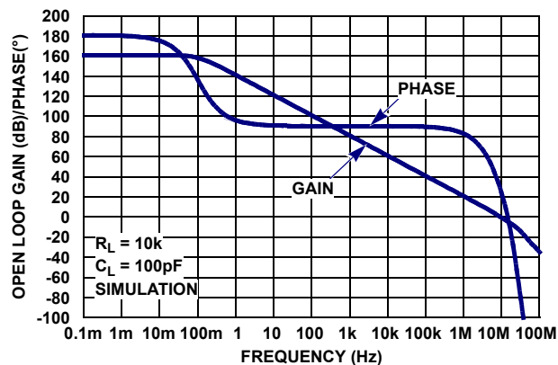
FIGURE 26. OPEN-LOOP GAIN, PHASE vs FREQUENCY, R_L = 10k\Omega , C_L = 100pF
