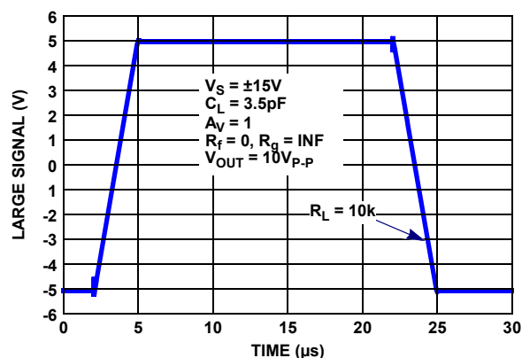
FIGURE 54. SIMULATED LARGE SIGNAL 10V STEP RESPONSE
