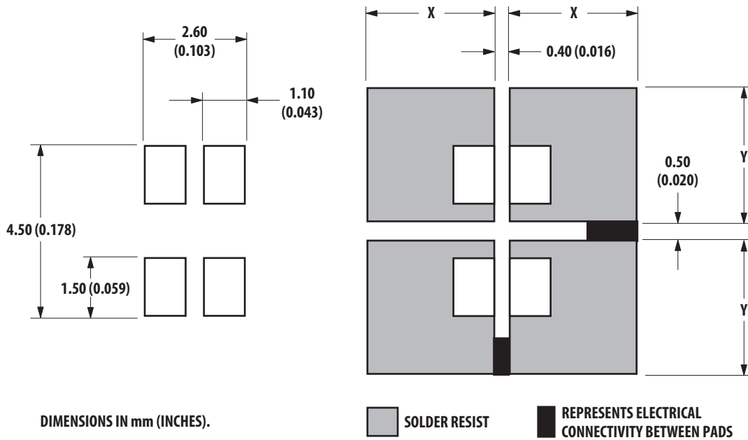
Figure 9: Recommended Soldering Pattern
