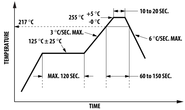
Figure 7: Recommended Pb-Free Reflow Soldering Profile
