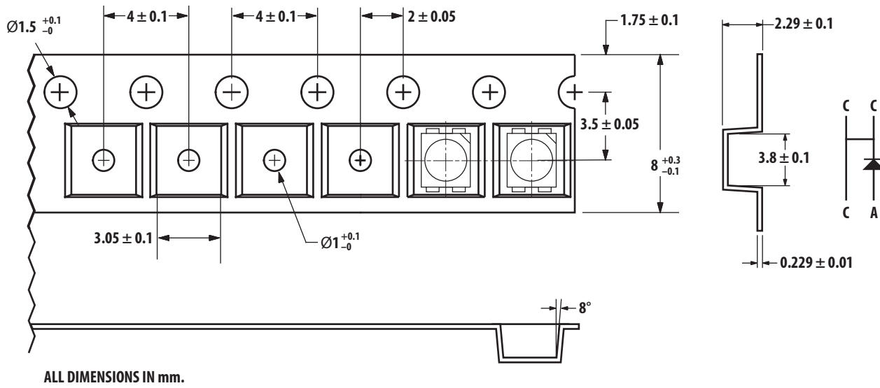
Figure 12: Reeling Orientation
