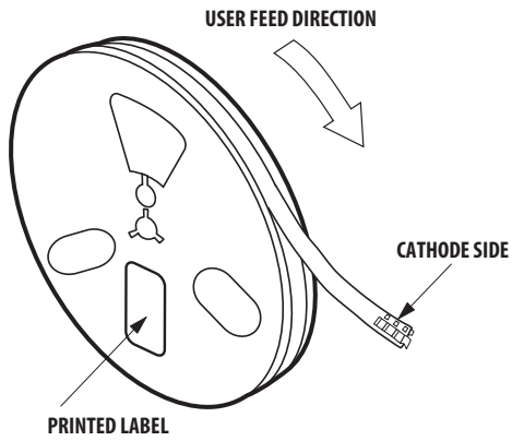
Figure 12: Reeling Orientation
