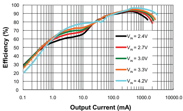
Efficiency (L = 2.2μH, V OUT = 5.0V)
