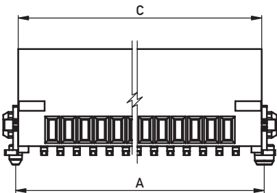
Unmated Stacking Height 3.25 mm
