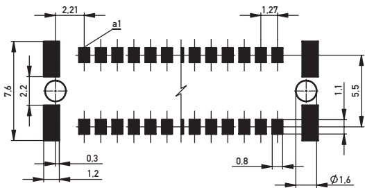
Recommended Layout
