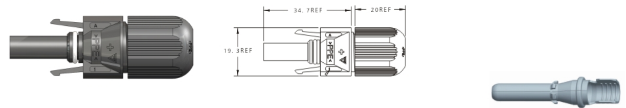
H4-RH Female Cable Connector
