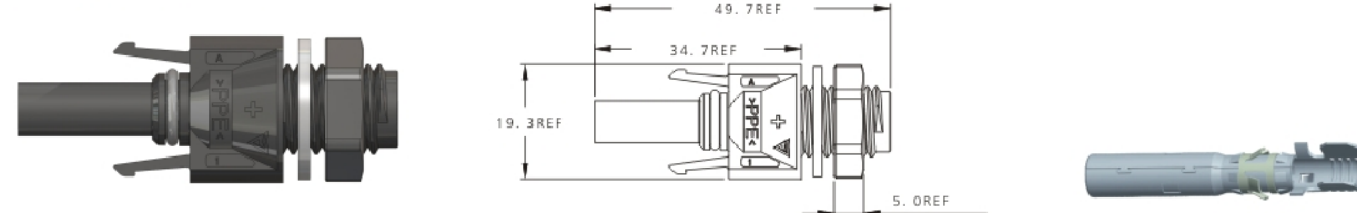
H4-R Female Panel Connector
