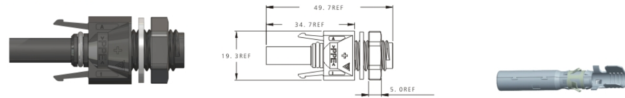
H4-RH Female Panel Connector
