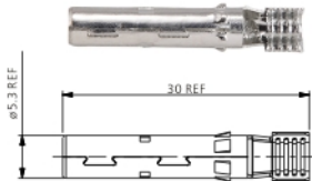
UTX™ Female socket contact
