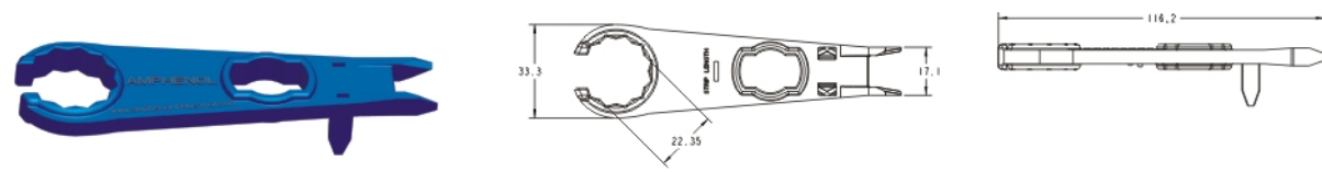
H4-XL connector wrench tool P/N: H4TW0004
