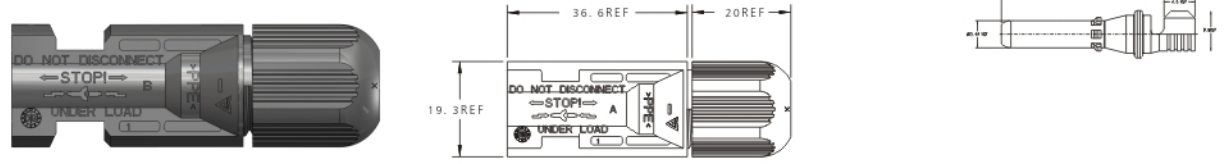
H4-RH Male Cable Connector
