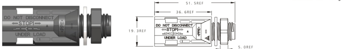
H4-R Male Panel Connector
