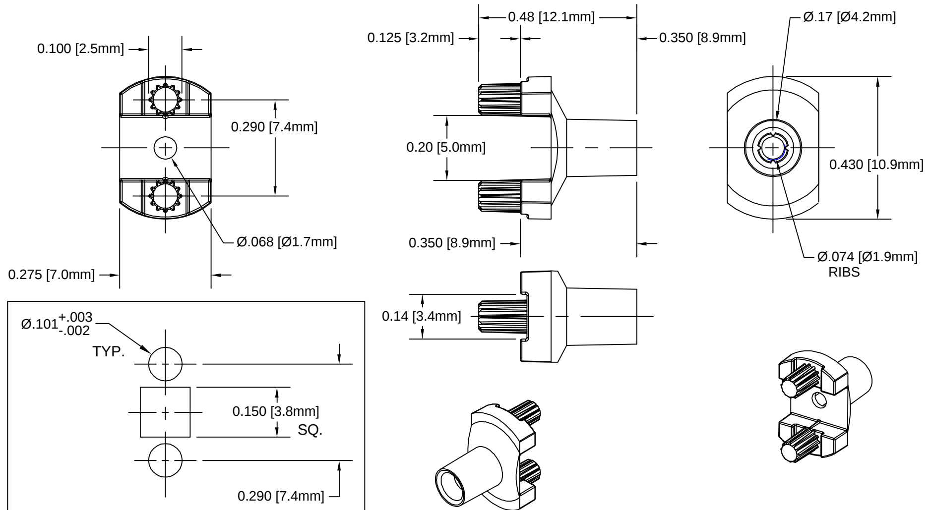
Recommended Soldering Pattern & Mounting Holes
