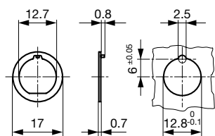
Transparent Cover 0853.0551
