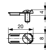
Screw-Adapter for Quick Connect-Terminals 6.3 x 0.8 mm
