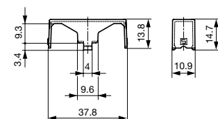
Reflow Cover
