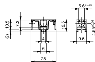
Reflow-Cover with Clamp 0853.0576
