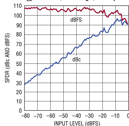
LTC2264-14: SFDR vs Input Level, f_{IN} = 70\text{MHz} , 2\text{V} Range, 40\text{Mpsps}
