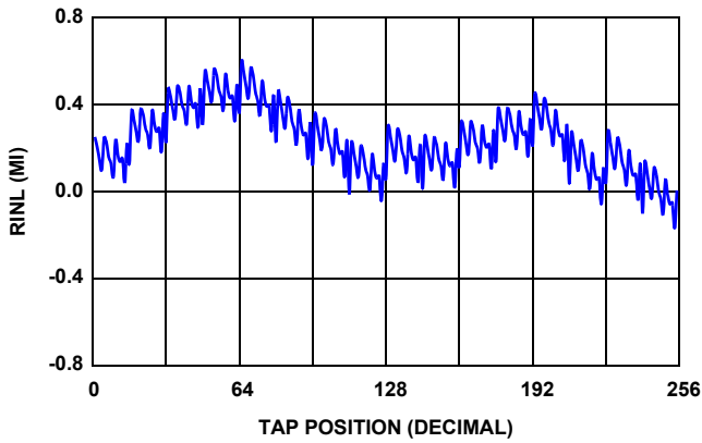
FIGURE 9. 10kΩ RINL vs TAP POSITION, V_{CC} = 3.3V , +25°C
