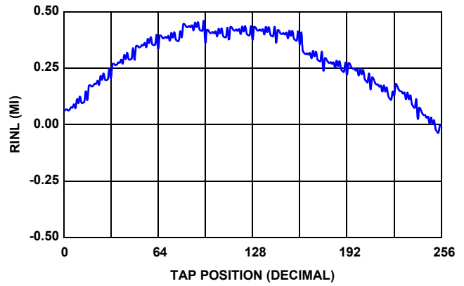
FIGURE 10. 50kΩ RINL vs TAP POSITION, V_{CC} = 3.3V , +25°C
