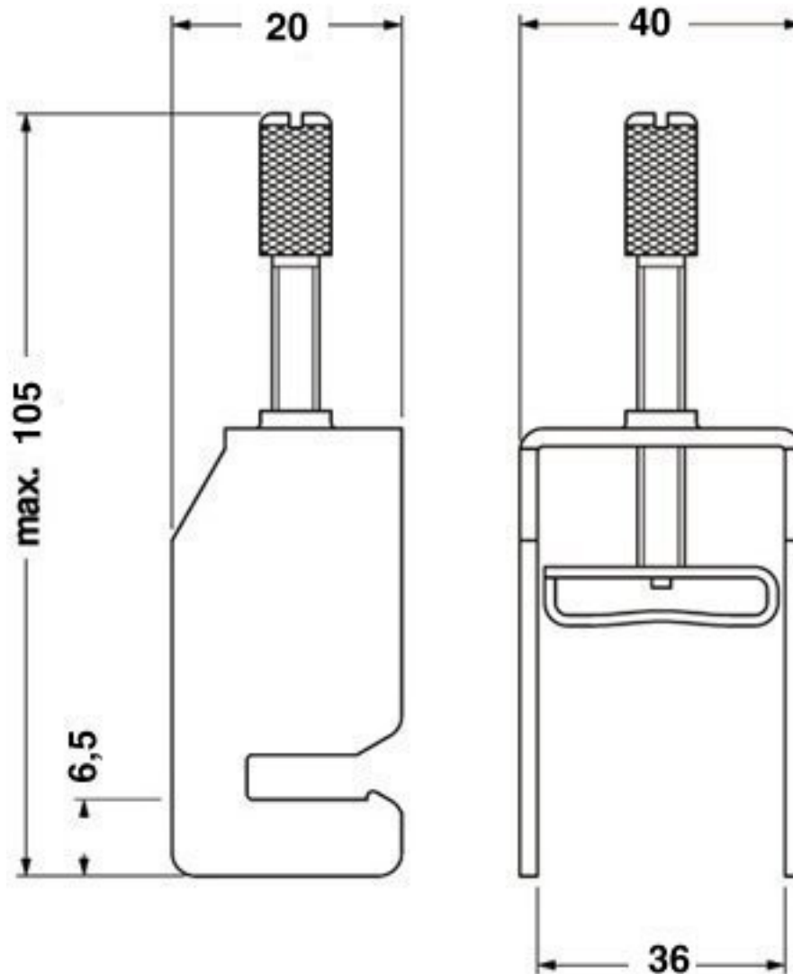
Dimensional drawing
