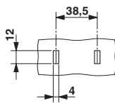
Dimensional drawing
