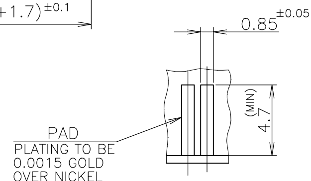
DETAIL G
