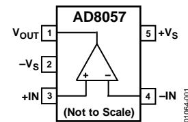
Figure 1. RT-5 (SOT-23)
