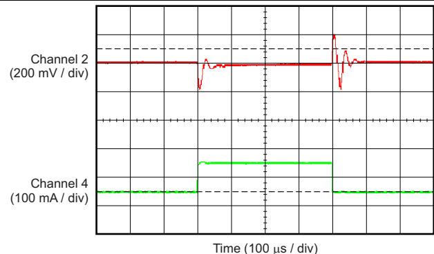
Figure 28. TPS70912-Q1 Load Transient (1 mA to 150 mA)
