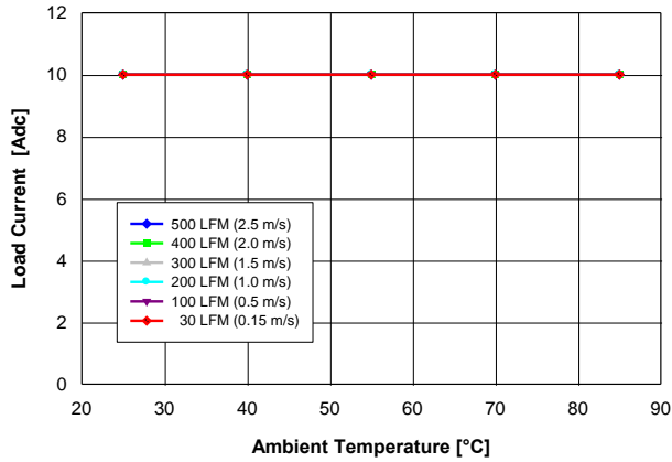
Fig. 1.0V.1: Available load current vs. ambient temperature and airflow rates for V_{out} = 1.0 V converter mounted vertically with V_{in} = 5 V, and maximum MOSFET temperature \leq 120 °C.
