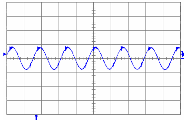
Fig. 3.3V.6: Output voltage ripple (20 mV/div.) at full rated load current into a resistive load with external capacitance 100\text{ }\mu\text{F} ceramic + 1\text{ }\mu\text{F} ceramic and V_{in} = 5\text{ V} for V_{out} = 3.3\text{ V} . Time scale: 2 \mu\text{s} /div.
