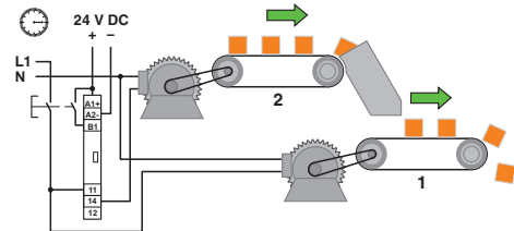
Conveyor belt 2 stars with a time delay
