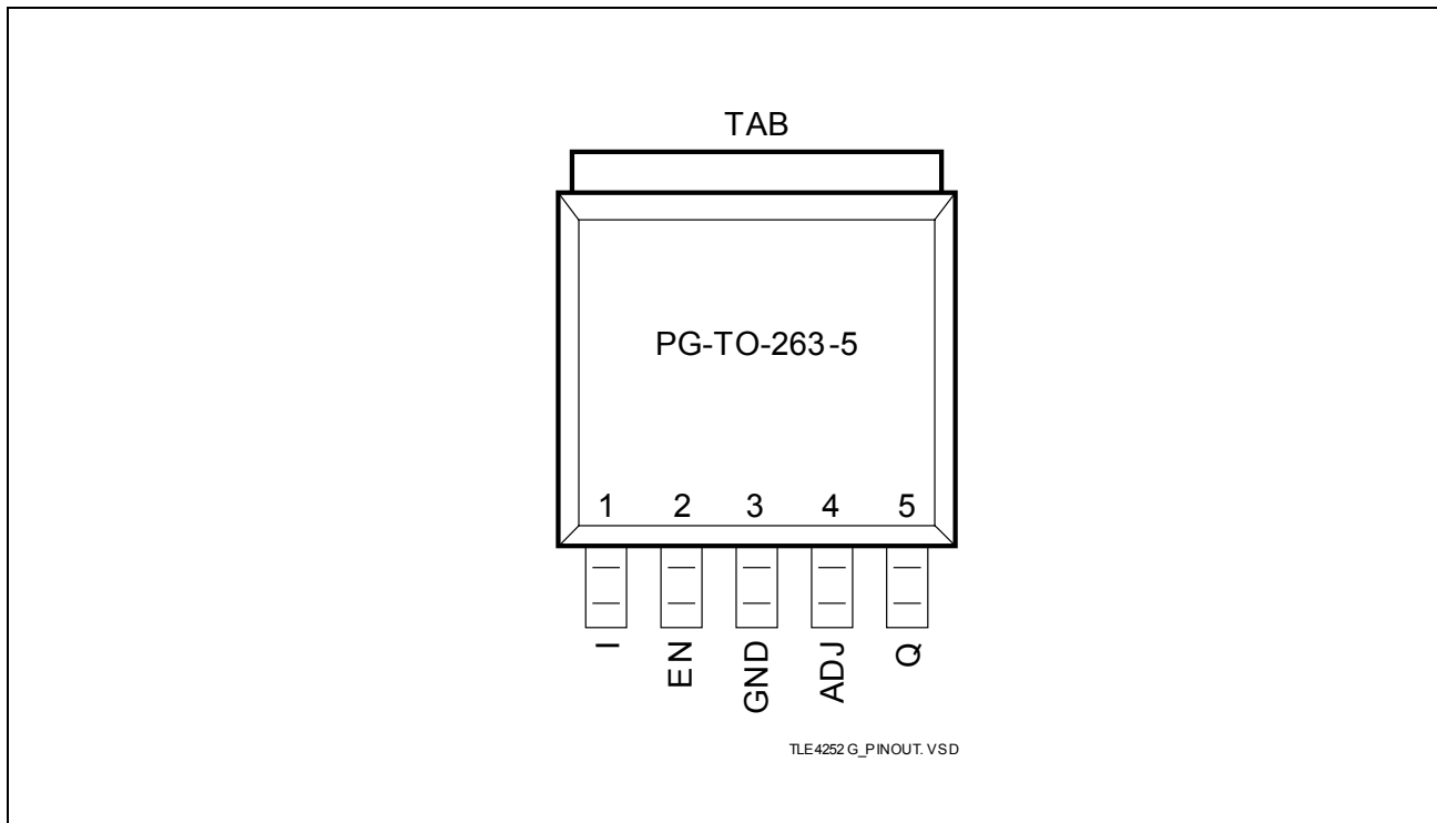
Figure 2 Pin Configuration
