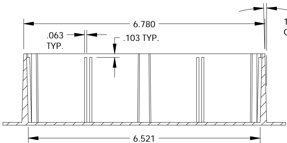
SECTION B-B
