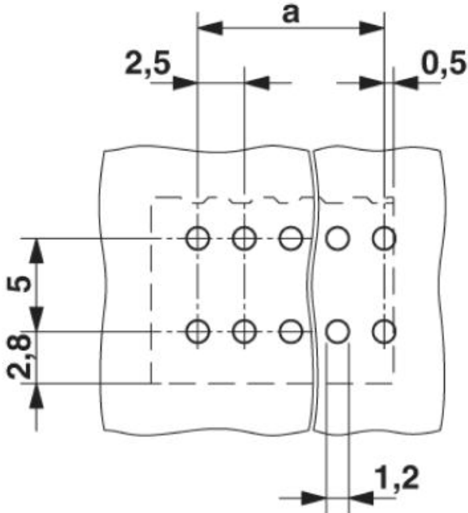
Drilling diagram
