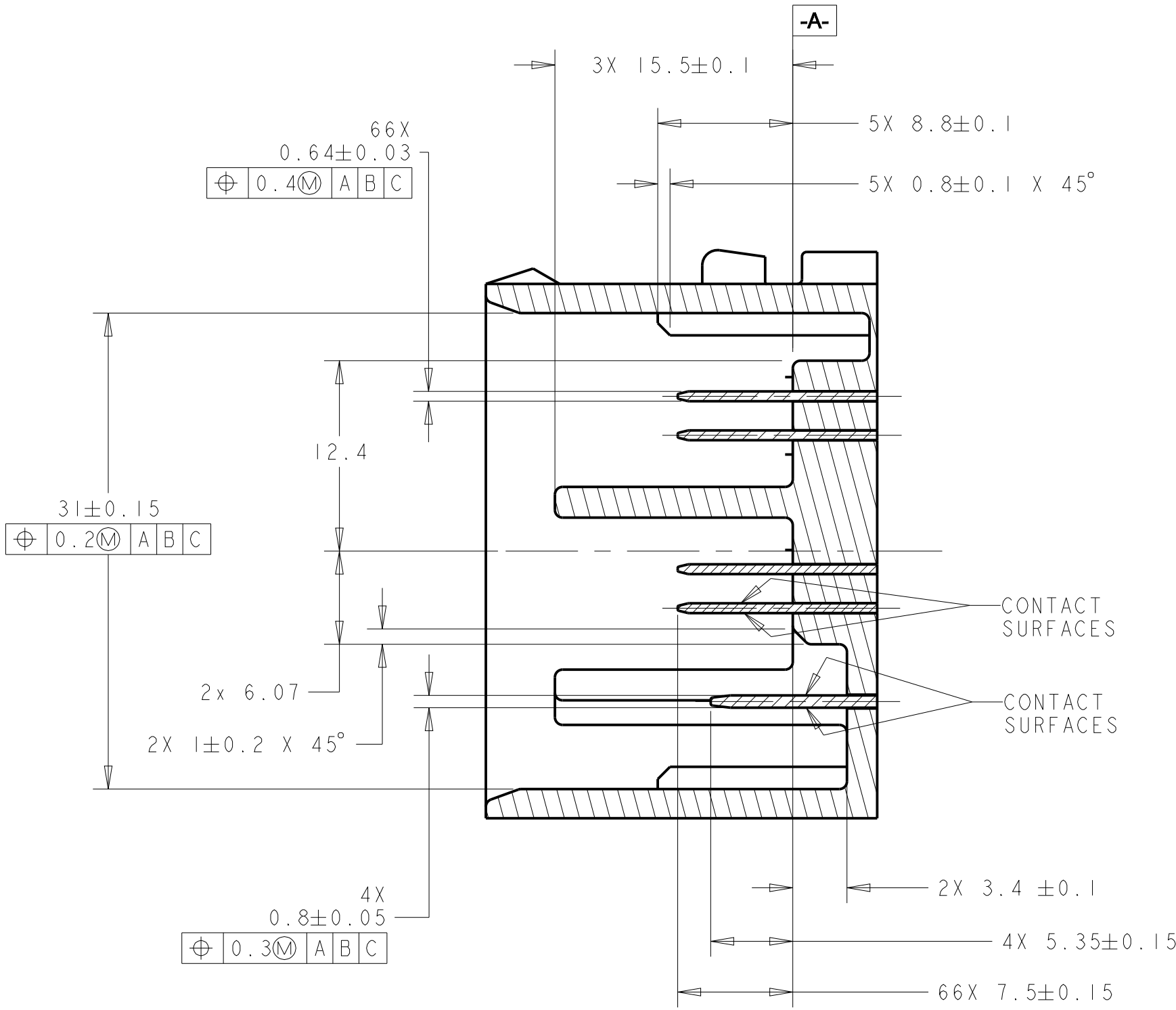
SECTION C-C
