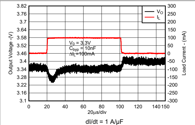
Figure 8-8. Load Transient Response for New Chip
