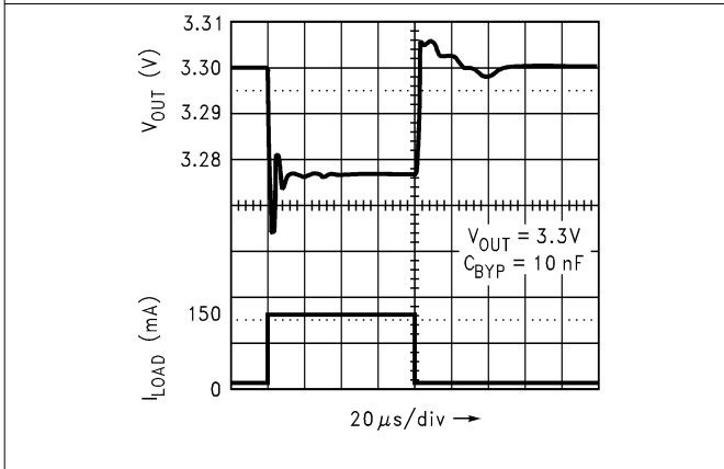
Figure 8-9. Load Transient Response for Legacy Chip
