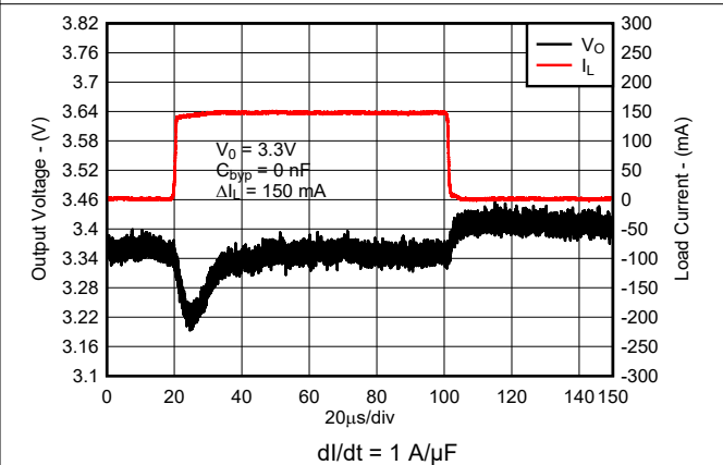
Figure 8-12. Load Transient Response for New Chip
