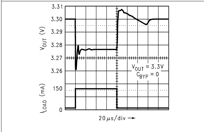
Figure 8-11. Load Transient Response for Legacy Chip
