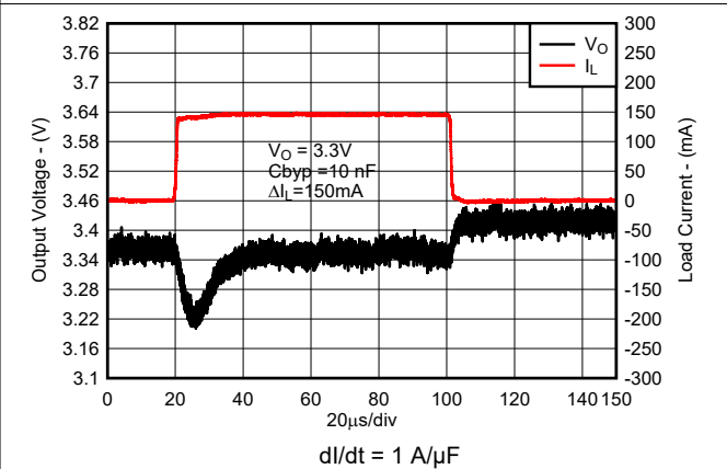
Figure 8-10. Load Transient for New Chip
