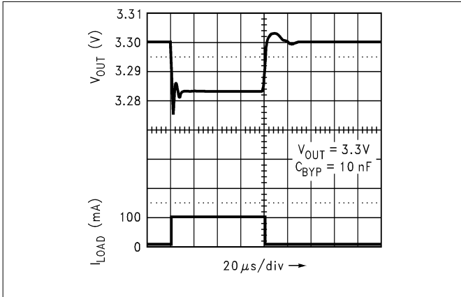
Figure 8-7. Load Transient Response for Legacy Chip
