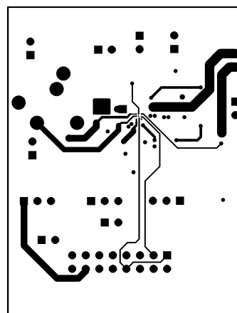
Figure 48. Bottom Layer
