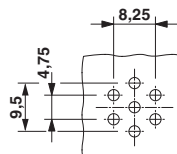
Drilling diagram
