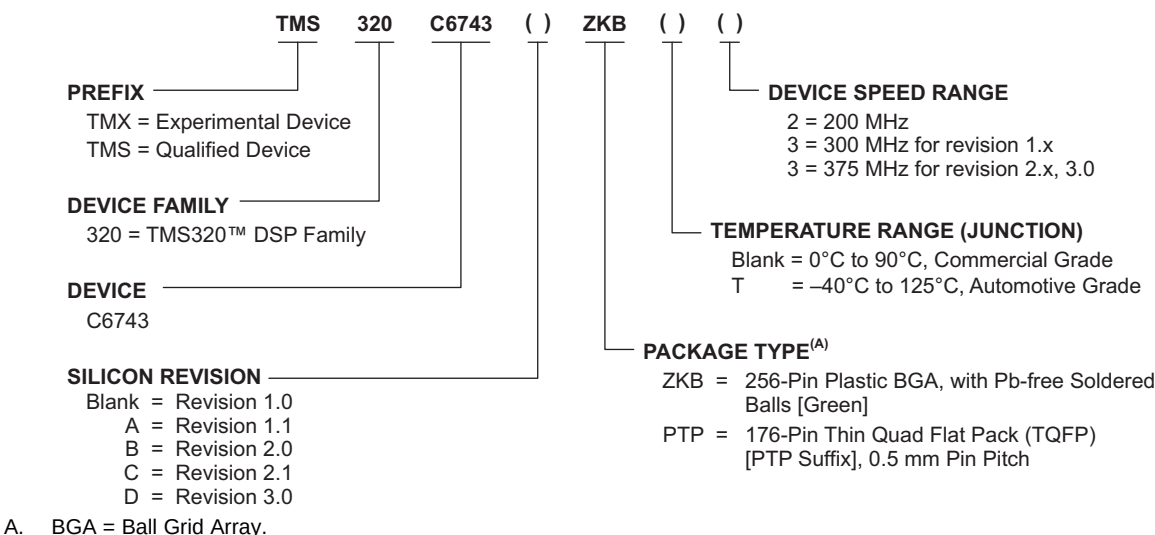
Figure 7-1. Device Nomenclature
