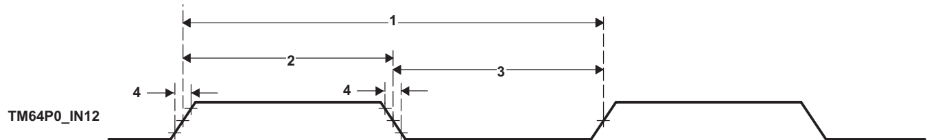
Figure 6-42. Timer Timing
