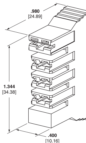
Part Number 521781-1 4-Position
