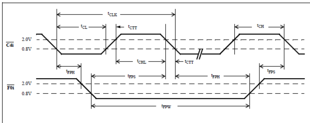
Figure 13 - Clock Timing
