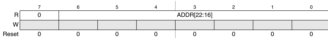
Figure 4-4. MPU Address Status Register 0 (MPUASTAT0)
