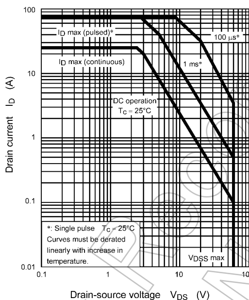
Fig. 8.14 Safe Operating Area (Guaranteed Maximum)
