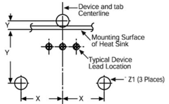
Mounting Details:
