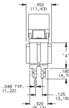
PC MOUNTING
