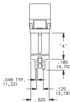
PC MOUNTING
