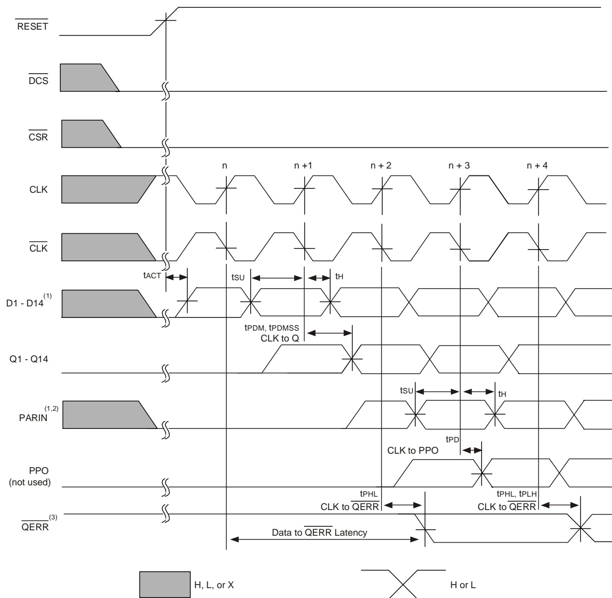
Timing Diagram for the Second SSTUBF32866B (1:2 Register-B Configuration) Device Used in a Pair; C0 = 1, C1 = 1, RESET Switches from L to H
