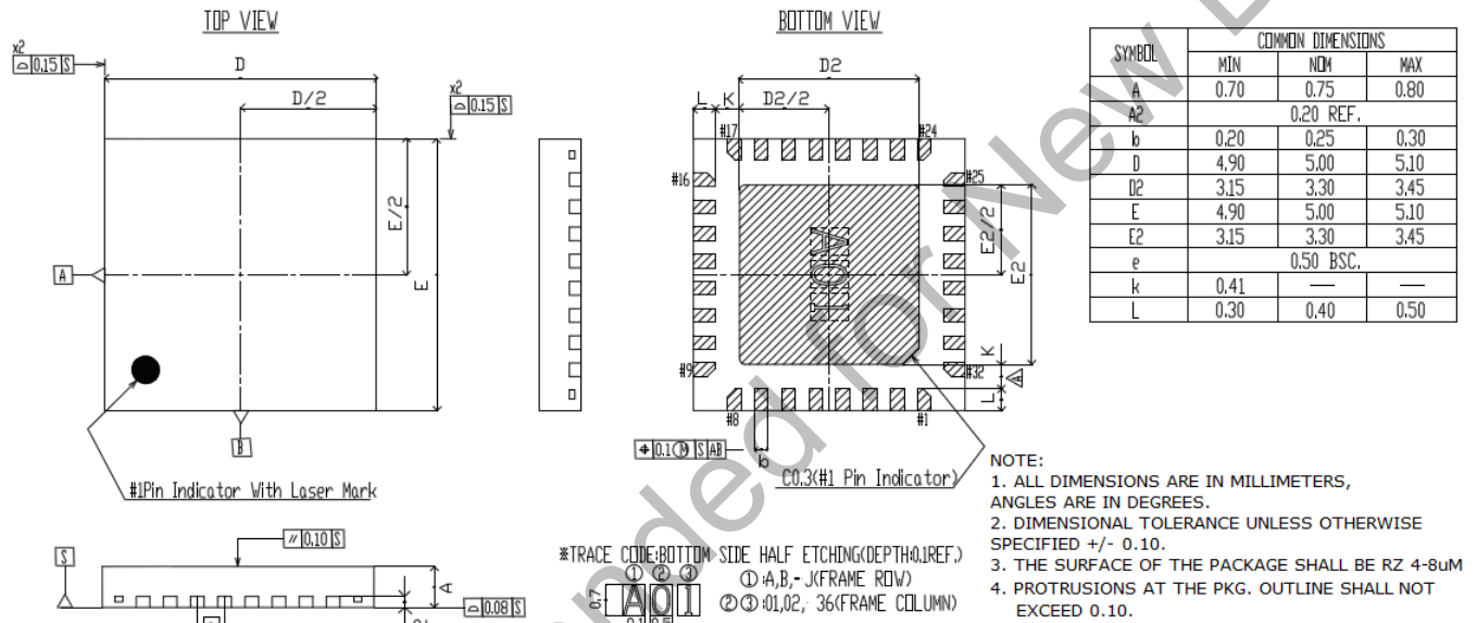
32-Lead QFN 5 x 5mm
