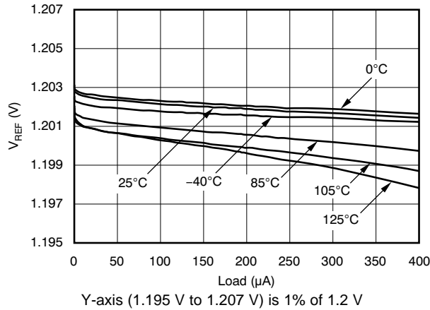
Figure 24. TPS386000-Q1 V_{REF} Output Load Regulation ( V_{DD} = 6.5\text{ V} )
