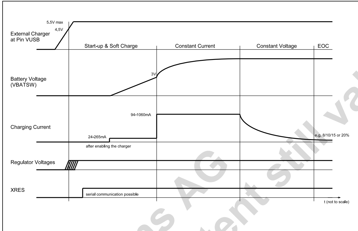
Figure 12. Charger States
