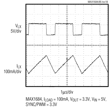
SWITCHING WAVEFORM
