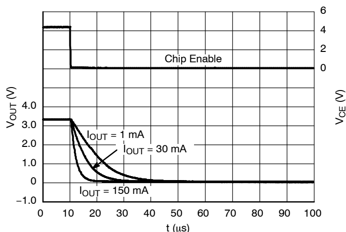
Figure 40. Shutdown, 3.3 V Version NCP4681D, V_{IN} = 4.3 V
