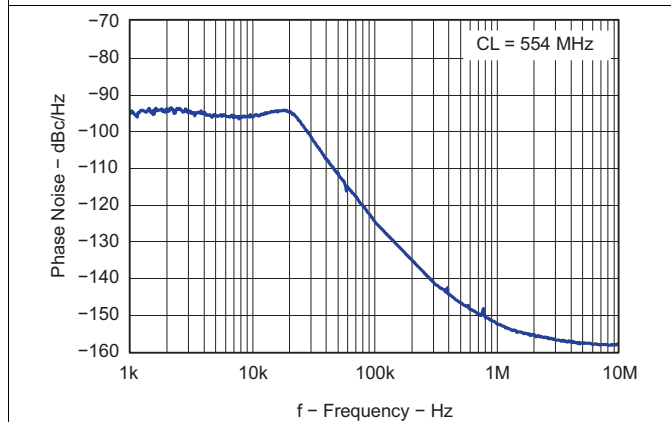
Figure 78. Closed Loop VCO Phase Noise
