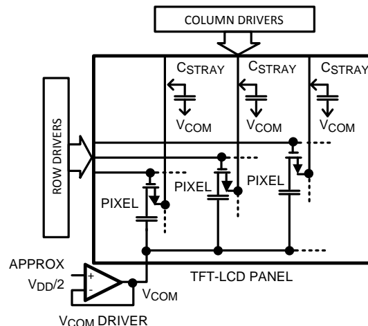
Figure 27. TFT Display
